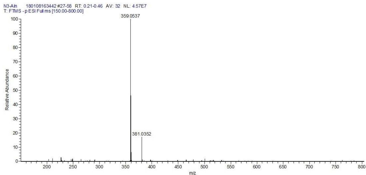
Figure S2. ESI-MS of N3-Alendronate (negative mode). Calculated: 360.06. Found: 359.05 (M-H), 381.04 (M-H+Na)
