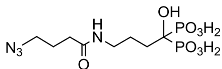
Figure S1. Structure of N3-Alendronate. Chemical Formula: C 8 H 18 N 4 O 8 P 2 ; Exact Mass: 360.0600; Molecular Weight: 360.1980
